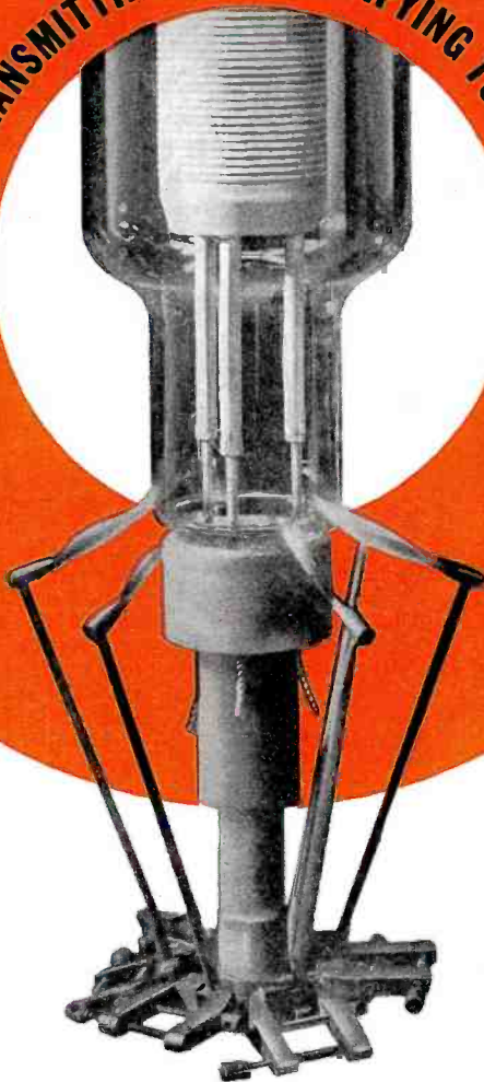
Photograph of sealing operation on vertical rotating fires of exclusive Amperex design.
